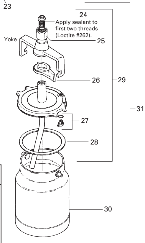
Figure 5 - Cup Drawing
